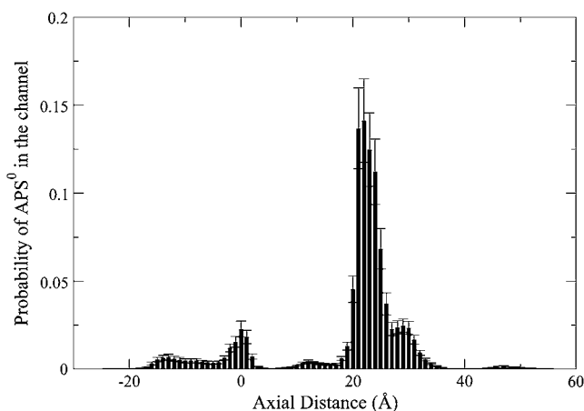
FIGURE 12 A dwell histogram indicates the region of the channel where the neutral ligands preferentially reside. The channel is divided into 80 sections, and the average probability in each slice is counted during 69 independent CGBD simulations of 2 \mu\text{s} . The standard deviation is represented with the line.
