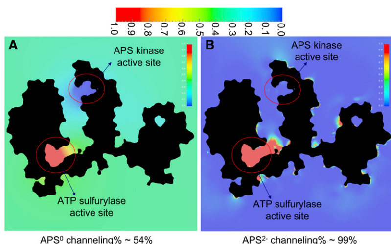
FIGURE 4 The intermediate concentration distribution in the solvent around SAC. Blue indicates extremely low concentration; cyan represents the medium low concentration and red the high concentration.
